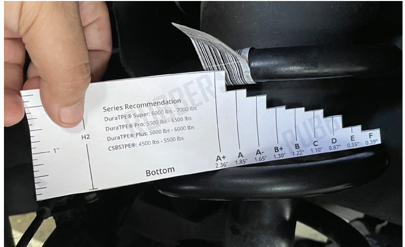
Choose size Buffer B + CSBPro-BP and Rubber Block RB275-2-175
